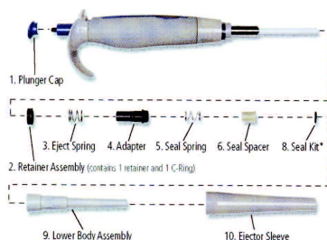
500 µL - 1 mL Pipettes
