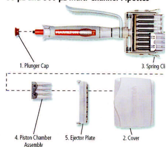
50 µL and 300 µL Multi-Channel Pipettes
